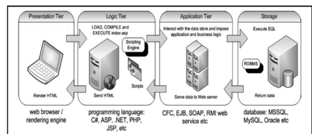
Figure 1. Database driven web application
