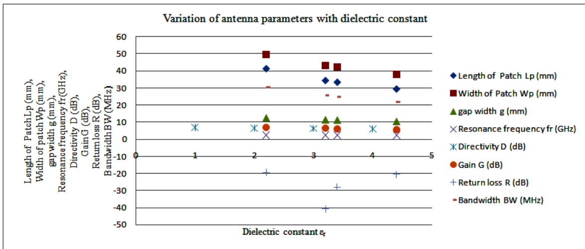
Fig. 2. Variation of antenna parameters with substrate material.
